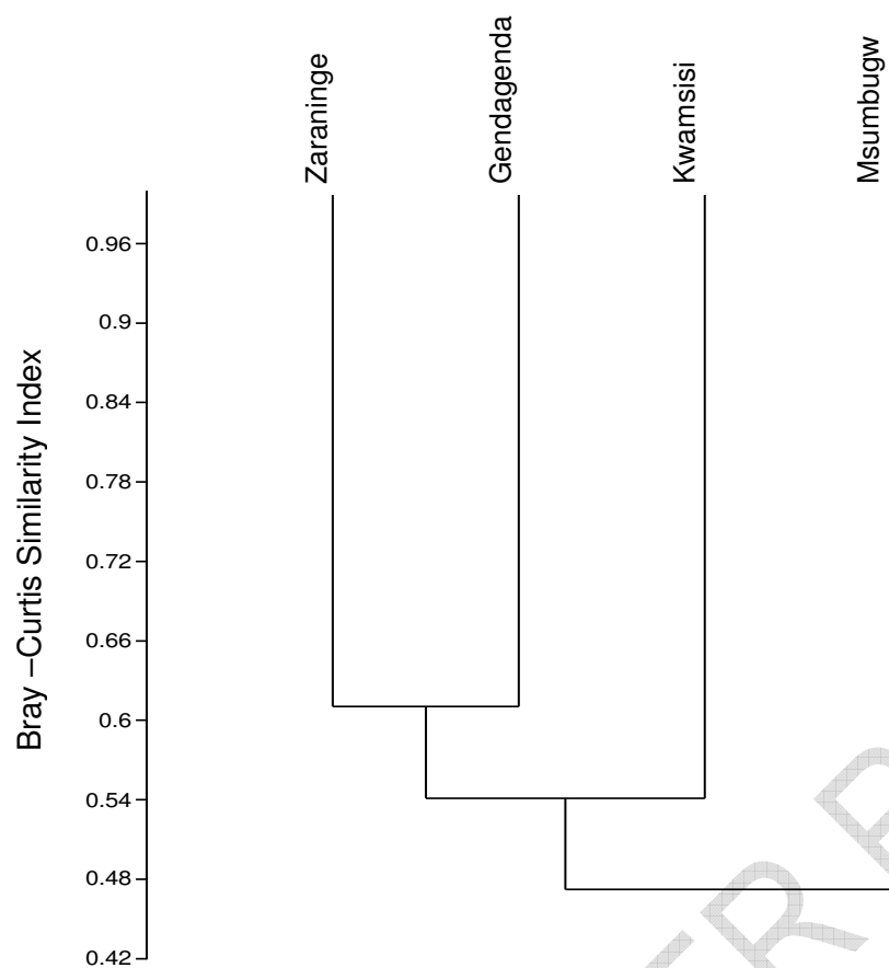
Figure 2: A Dendrogram showing similarity in bird species composition in the four forests in Pangani-Saadani ecosystem from data collected during October 2010 to January 2011.
